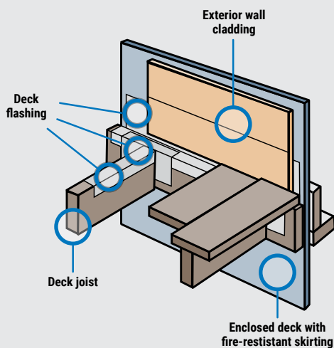
Figure 16: Deck flashing
